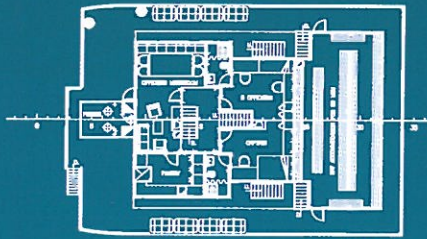
OFFICER'S DECK
