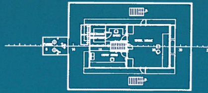
WHEEL HOUSE DECK
